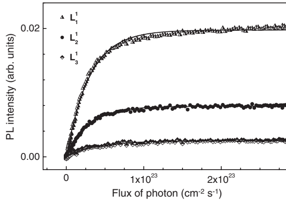
Figure 2. PL intensity dependence on the excitation photon flux for the three major lines L_1^1 , L_2^1 and L_3^1 measured at T = 4.2 K under pulsed excitation with the OPO set to \lambda_{\text{exc}} = 520 nm.
