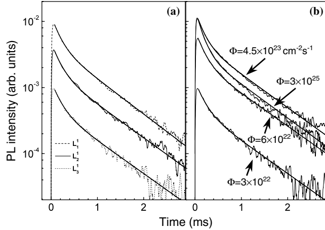
Figure 3. PL decay dynamics measured at T = 4.2 K under pulsed excitation with the OPO set to \lambda_{\text{exc}} = 520 nm for (a) the three major lines L_1^1 , L_2^1 and L_3^1 with \Phi = 3 \times 10^{22} \text{cm}^{-2} \text{s}^{-1} photon flux and (b) the L_1^1 line at several different photon flux values.
