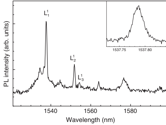
Figure 1. Photoluminescence spectrum of the multilayer sample used in the current study as obtained at T = 4.2 K under pulsed excitation with the OPO set to \lambda_{\text{exc}} = 520 nm. In the inset: the ultranarrow linewidth of the main emission band L_1^1 measured at T = 4.2 K under cw excitation with an \text{Ar}^+ ion laser ( \lambda_{\text{exc}} = 514 nm).
